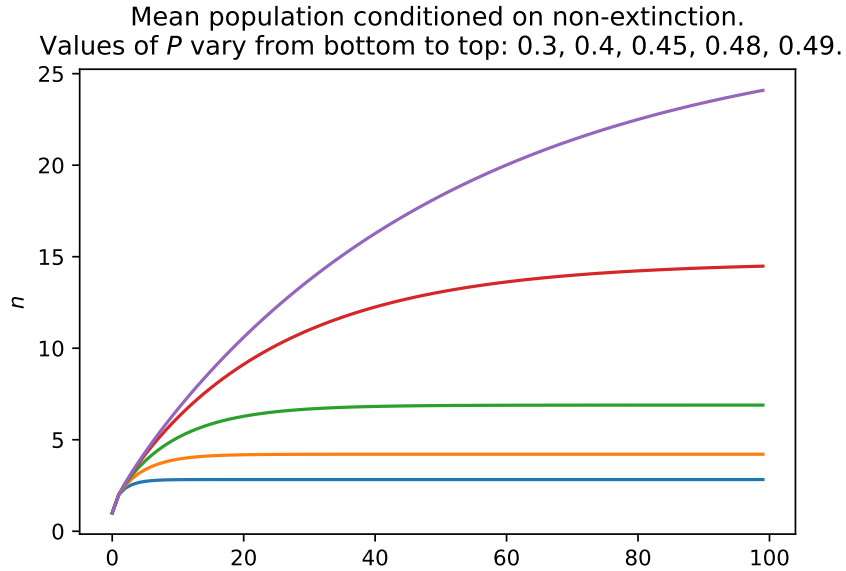
Figure 1.9: The conditional mean (2p)^n/S_n against generation number n , with S_n obtained by iterating (1.11). From bottom to top, p = 0.3, 0.4, 0.45, 0.48, 0.49 . Each curve approaches the constant 1/A(p) ; the limiting values are 2.825, 4.208, 6.893, 14.703 and 27.476. The lowest three have essentially converged by n = 100 , but the p = 0.49 curve has reached only 24.1 of its limiting 27.5 — an early sign of a near-critical slowdown that the following chapter analyses and works around.
