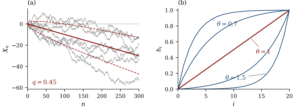
Figure 1.1: The simple random walk of (1.2). (a) Seven realisations at q = 0.45 (grey), against the drift line n(2q - 1) and the envelope \pm\sqrt{4nq(1 - q)} of one standard deviation (red), from (1.3). The drift is linear in n and the spread only O(\sqrt{n}) , so the drift eventually dominates; over the first hundred steps it does not, and individual paths spend long intervals on the wrong side of the mean. (b) The gambler's-ruin probability (1.5) of reaching M = 20 before 0, against the starting state i , for \theta = (1 - q)/q \in \{0.7, 0.85, 1, 1.2, 1.5\} . The symmetric case \theta = 1 is the straight line i/M ; \theta < 1 bows the curve up and \theta > 1 bows it down, and the effect is strongly nonlinear in \theta . Only the ratio \theta enters, which is why (1.51) can read this figure off the embedded jump chain of a birth–death process without reference to its rates.
