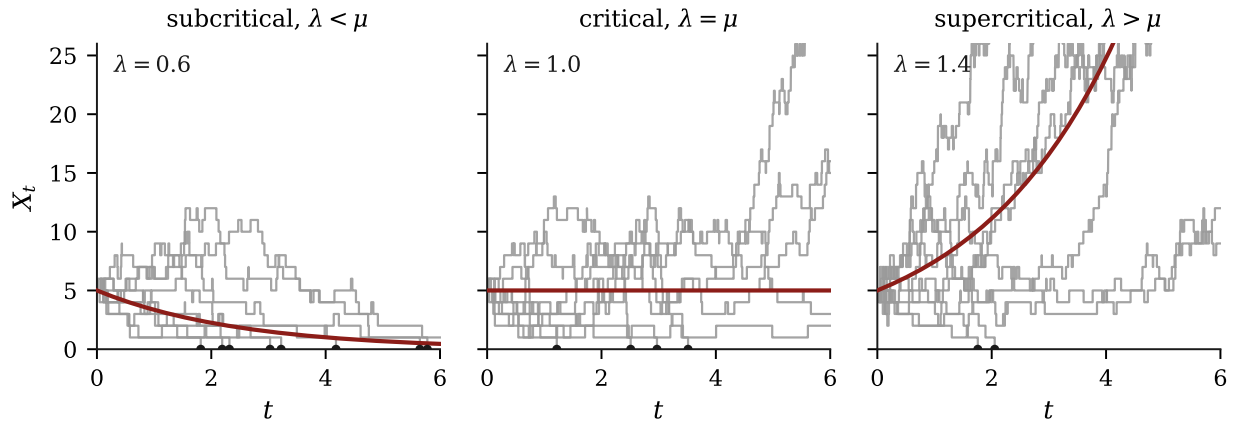
Figure 1.4: Nine realisations of the linear birth–death process (1.20) from X_0 = 5 , with \mu = 1 throughout and the mean Ne^{(\lambda-\mu)t} of (1.47) in red; dots on the axis mark trajectories that reached the absorbing state. The middle panel is the one to dwell on. At criticality the mean is exactly constant, and yet several realisations are already extinct while others have grown fourfold — the mean is the same number in both cases, and describes neither. That gap between a mean and a distribution is what the conditioning of section 1.3.2.6 exists to close. Note also that extinction is not confined to the subcritical panel: a supercritical process still dies out with probability (\mu/\lambda)^N , visible here as the paths that fail early on the right.
