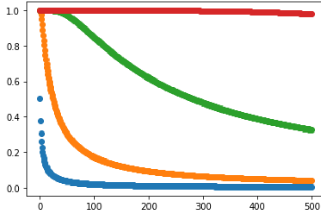
Figure 1.17: Survival probability S_n^{(k)} from (1.88) out to 500 generations at exact criticality, p = 0.5 , for k = 1, 10, 100, 1000 (blue through to red). A larger founding cohort buys longevity, but at criticality every curve is still headed for zero.
