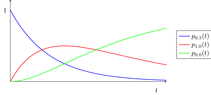
Figure 1.13: State probabilities for the single-particle absorption–death model, (1.69). The particle starts outside ( p_{0,1} , blue), is absorbed into the compartment ( p_{1,0} , red, which rises and then decays as death takes over), and finally dies ( p_{0,0} , green, absorbing).
