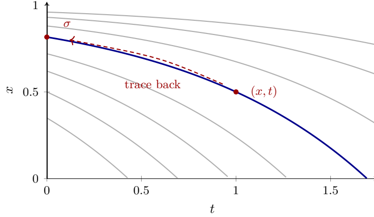
Figure 1.11: Characteristics of the x -equation (1.73), dx/d\tau = \mu(1 - x) with \tau = -t , drawn for \mu = 1 . Each grey curve is one characteristic, x(t) = 1 - (1 - \sigma)e^{\mu t} , labelled by the point \sigma at which it meets the initial surface t = 0 , drawn as the heavy vertical line; together they foliate the domain, and exactly one passes through any given (x, t) . Since G is constant along characteristics, its value at a point is its value at the foot of that point's curve — so solving the equation amounts to running the curve backwards from (x, t) to t = 0 and reading off \sigma , here \sigma = 1 - (1 - x)e^{-\mu t} . The full problem is three-variate; this is its projection onto the (x, t) plane, which is where the cascade starts, because (1.73) does not involve y .
