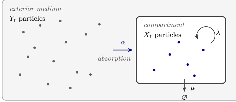
Figure 1.12: The single-compartment absorption models. Particles begin in the exterior medium and are taken up one at a time, each independently at rate \alpha , so the absorption channel carries total rate Y_t\alpha ; once inside, a particle dies at rate \mu and, in the fullest version of the model, divides at rate \lambda . Only the three transitions drawn here occur, and each is proportional to the count in the compartment it acts on — which is what makes the generating-function equation first order and puts it within reach of section 1.3.3.1 . Switching channels off gives the family in order of difficulty: with \lambda = \mu = 0 the particles are merely relocated ( section 1.B.1 ); with \lambda = 0 this is the worked example below; with all three active the interior state space becomes infinite and section 1.B.2 must solve the equation directly. Note that nothing returns from the compartment to the medium, which is why the exterior count is unaffected by the interior dynamics.
