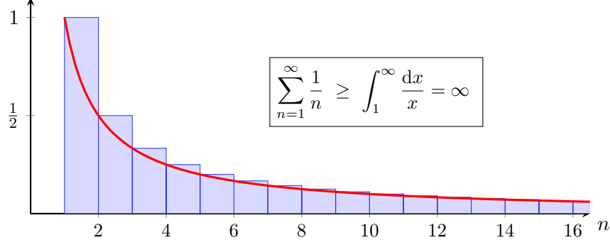
Figure 1.14: Divergence of the harmonic series. Each blue rectangle has area 1/n and contains the region under the red curve 1/x on [n, n+1] , so the sum of the areas exceeds \int_1^{\infty} x^{-1} dx = \infty . Because S_n \sim 2/n at criticality, the same divergence carries over to \mathbb{E}(T) = \sum_n S_n .
