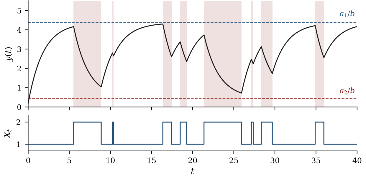
Figure 1.6: A trajectory of a coupled ODE–CTMC system of the two-way form (1.30). The continuous variable follows dy/dt = a(X_t) - by , so it relaxes towards a_1/b while X_t = 1 and towards a_2/b while X_t = 2 (dashed lines); the chain switches 1 \rightarrow 2 at rate \kappa y , which depends on the continuous state, and back at a constant rate. Upper panel: y(t) , with the intervals spent in state 2 shaded. Lower panel: the discrete component X_t . The visits to state 2 concentrate where y is large, which is the y -dependence of the rate made visible; the resulting descents then remove the very condition that made them likely. The joint process (y(t), X_t) is Markov although neither component is, and its generator is (1.31). The parameters are illustrative only.
