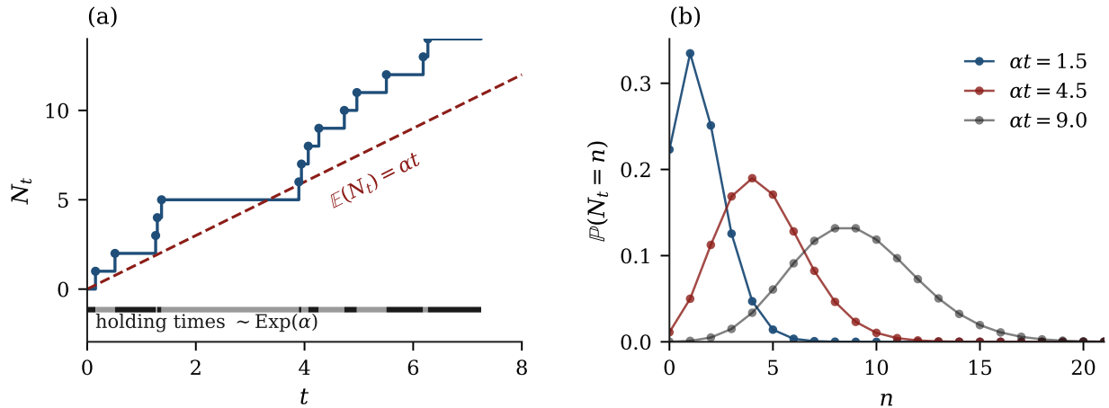
Figure 1.3: The Poisson process of (1.18), at rate \alpha = 1.5 . (a) One realisation of the counting process N_t , with the independent \text{Exp}(\alpha) holding times of proposition 1.1 marked in alternating shades along the axis, and the mean \alpha t dashed. The path crosses and recrosses its own mean; nothing prevents a long wait followed by three arrivals in quick succession, because each holding time is drawn afresh. (b) The law (1.19) at t = 1, 3, 6 . Mean and variance are both \alpha t , so the distribution broadens as it advances and its relative width 1/\sqrt{\alpha t} shrinks.
