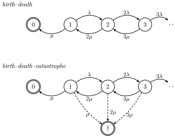
Figure 1.5: Transition-rate diagrams for the linear birth–death process (1.20) and for the birth–death–catastrophe process of definition 1.3 . Double circles mark absorbing states. Every rate is proportional to the current count, because individuals act independently. The two differ in one structural respect: the birth–death chain can only be absorbed by stepping down through state 1, whereas catastrophe (dashed) removes the population from any state in a single transition, and does so faster the fuller the compartment is. That is why survival mass drains from state 1 alone in the first process but from every positive state in the second, as (1.24) records, and it is what makes \dagger and 0 genuinely different endings rather than two labels for extinction.
