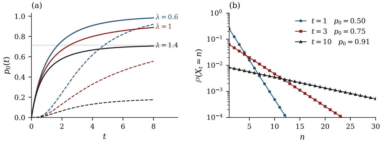
Figure 1.8: (a) The extinction probability (1.52) against time, with \mu = 1 and \lambda = 0.6, 1, 1.4 ; solid curves start from N = 1 , dashed from N = 5 . Below and at criticality every curve climbs to one, however large the founding cohort; above it the curves level off at (\mu/\lambda)^N , marked dotted for N = 1 , and a larger cohort buys a permanently smaller extinction probability rather than merely a delay. (b) The critical case in detail, from one founder: the law of X_t on the positive states at t = 1, 3, 10 , on a logarithmic scale. Absorbing mass accumulates at zero — p_0 rises from 0.50 to 0.91 — while the surviving tail flattens and stretches. The mean is exactly 1 at all three times. Neither the growing chance of extinction nor the lengthening tail is visible in that number, which is the sense in which the mean of (1.47) answers the wrong question.
