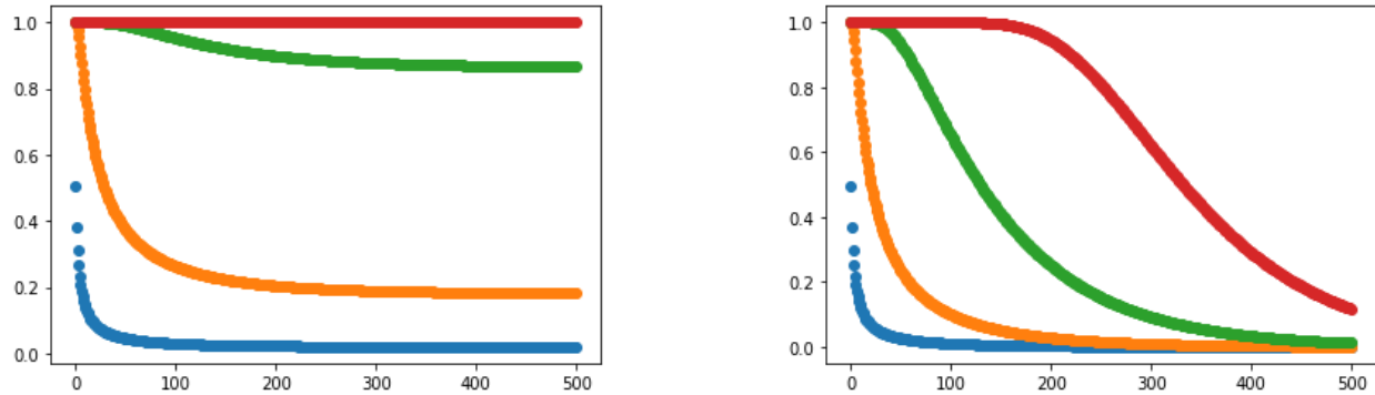
Figure 1.18: As figure 1.17 , but with p displaced slightly from criticality: p = 0.505 on the left (supercritical), p = 0.495 on the right (subcritical). A displacement of half a per cent separates curves that were nearly coincident in figure 1.17 .
